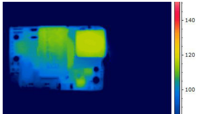
Figure 4. Thermal Image of CPT4B48 (4.2A output, 85C Ambient, 200lfm airflow, Vin = 48V, airflow from pin 3 to pin 1, T max = 119°C)
