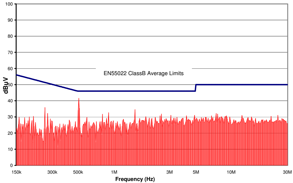
Figure 18. CPT4B48 Conducted Emissions using above specified input filter. Vin = 48V, Full Resistive Load
