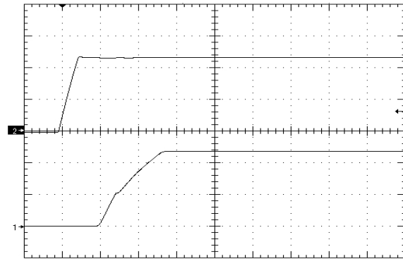
Figure 10. Startup Waveform via Line Voltage, time scale 10mS/div. Vin=Vin_nom, full resistive load + 2200uF. Ch1=5V/div, Ch2=5V/div
