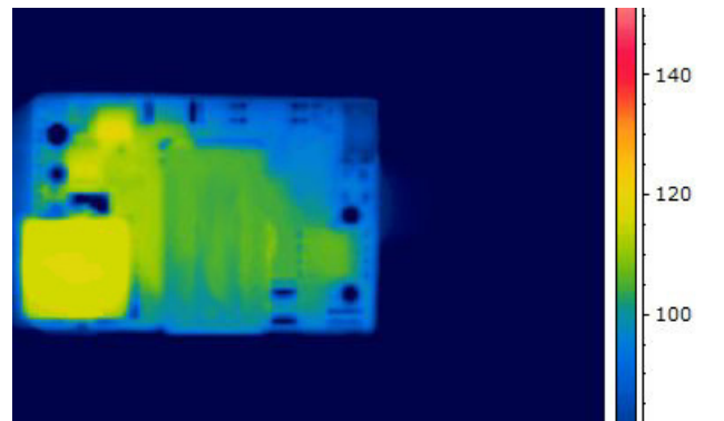
Figure 6. Thermal Image of CPT4B48 (4.2A output, 85C Ambient, 200lfm airflow, Vin = 48V, airflow from pin 1 to pin 3, T max = 122°C)
